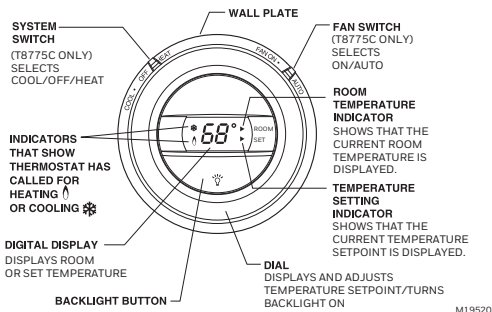
Fig. 10. T8775 Thermostat (features and operation).
